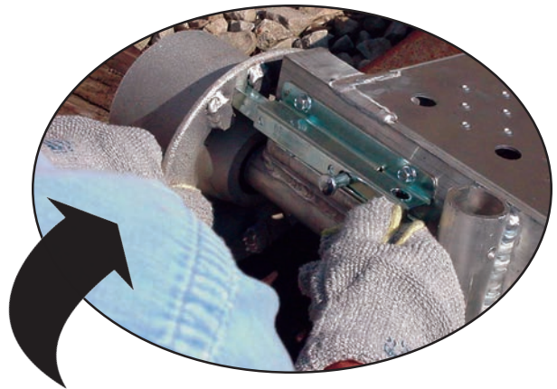
Setting the parking brakes, located on both ends of the cart, is fast and easy, locks the wheels, and secures and stabilizes the cart on track grades and during loading and unloading.
